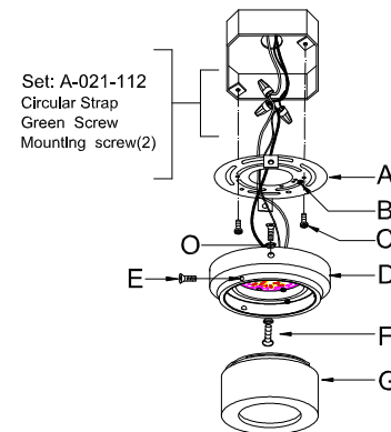
Fig.2 Ceiling Mount
